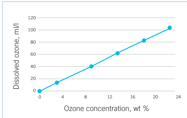
Amount of dissolved ozone is directly proportional to the ozone concentration at any given temperature (here 10°C).
